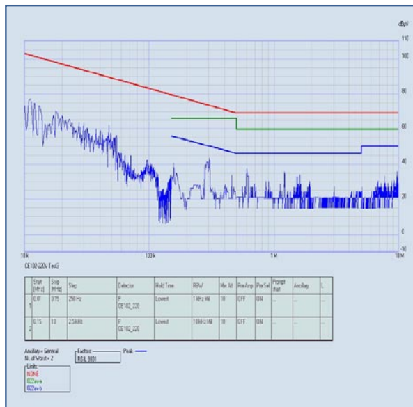
Example of EMI emission powerPAC4K 5V-150A, 3V3-135A, +12V-8A @230Vac/50Hz
