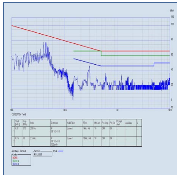
Example of EMI emission powerPAC4K 5V-150A, 3V3-135A, +12V-8A @115Vac/50Hz
