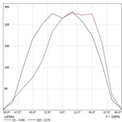
Illumination Curve
