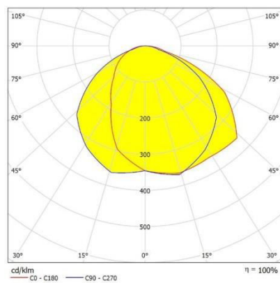
Luminance Distribution
