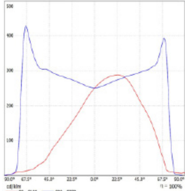
Illumination Curve
