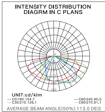
Lighting Distribution
