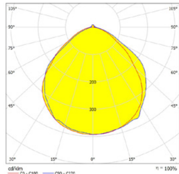
Lighting Distribution
