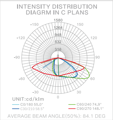
Lighting Distribution
