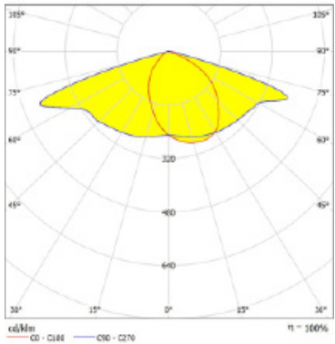
Luminance Distribution
