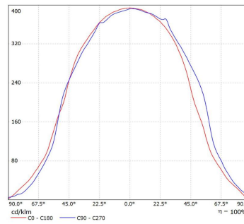
Illumination Curve
