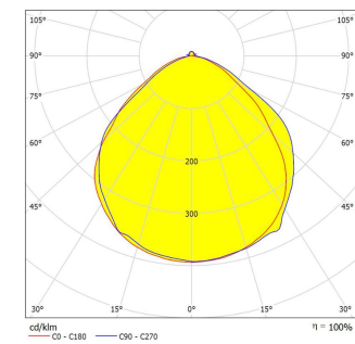
Luminance Distribution
