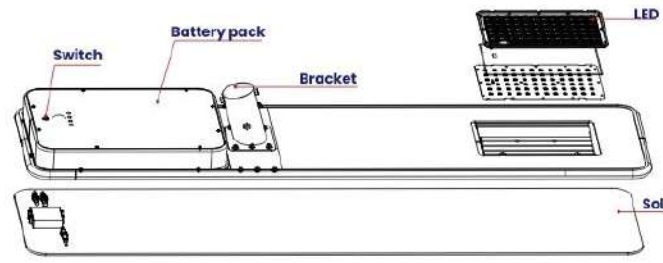
For Φ60mm pole Rust Proof bracket
