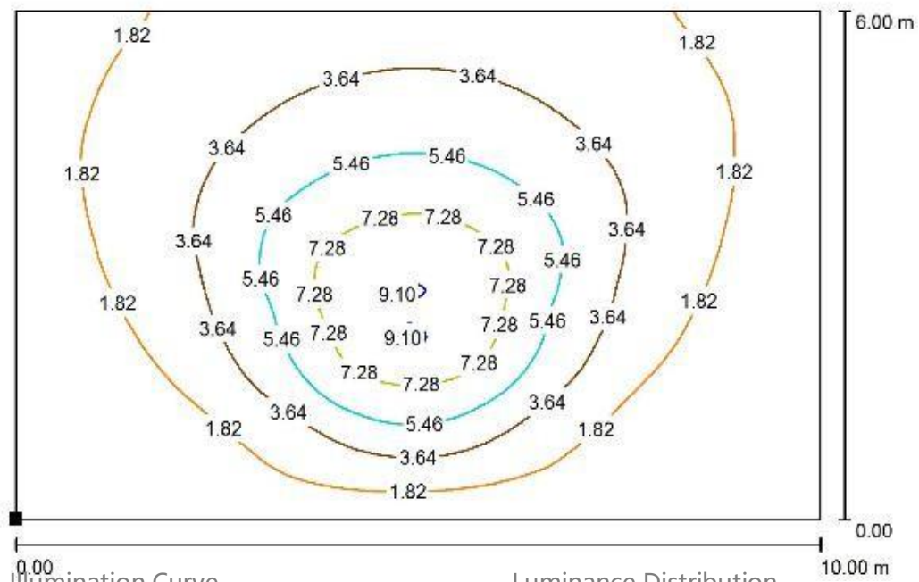
Illumination Curve
