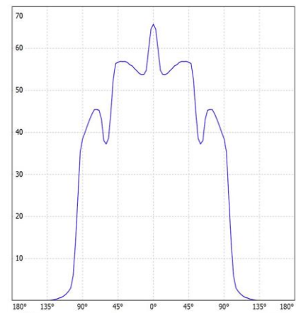
Luminance Distribution
