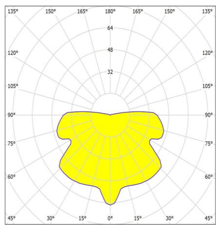
Illumination Curve
