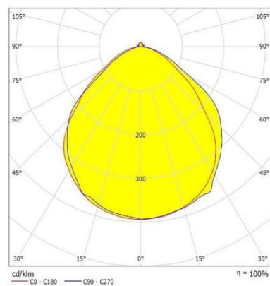
Luminance Distribution
