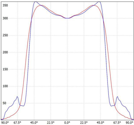
Luminance Distribution
