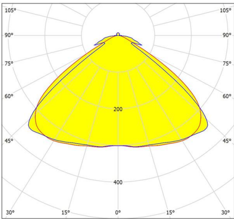
Illumination Curve
