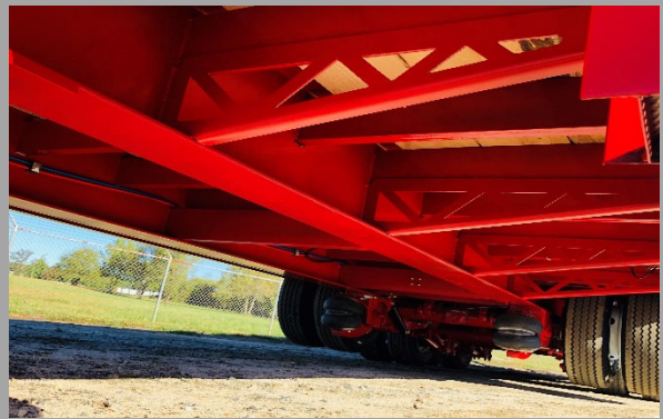
14" I-BEAM W/ PIERCED CROSSMEMBERS HD FORMED CROSSMEMBER GUSSETS
