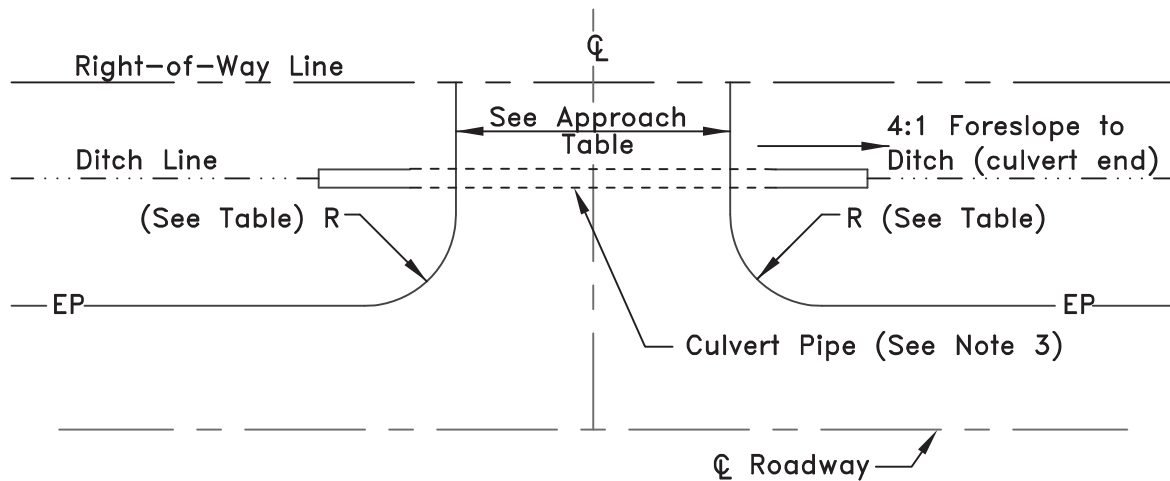
APPROACH PLAN
