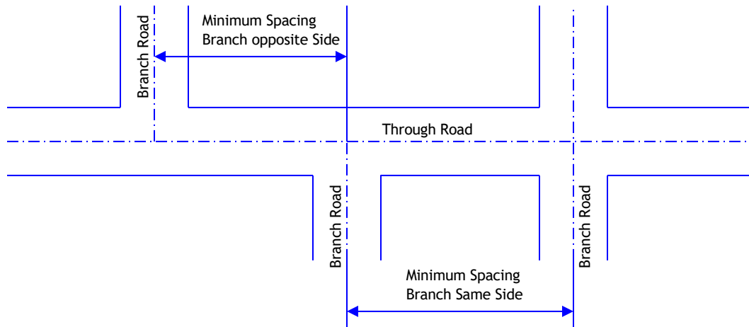
A. Rural Roadway Spacing (see spacing diagram above):
