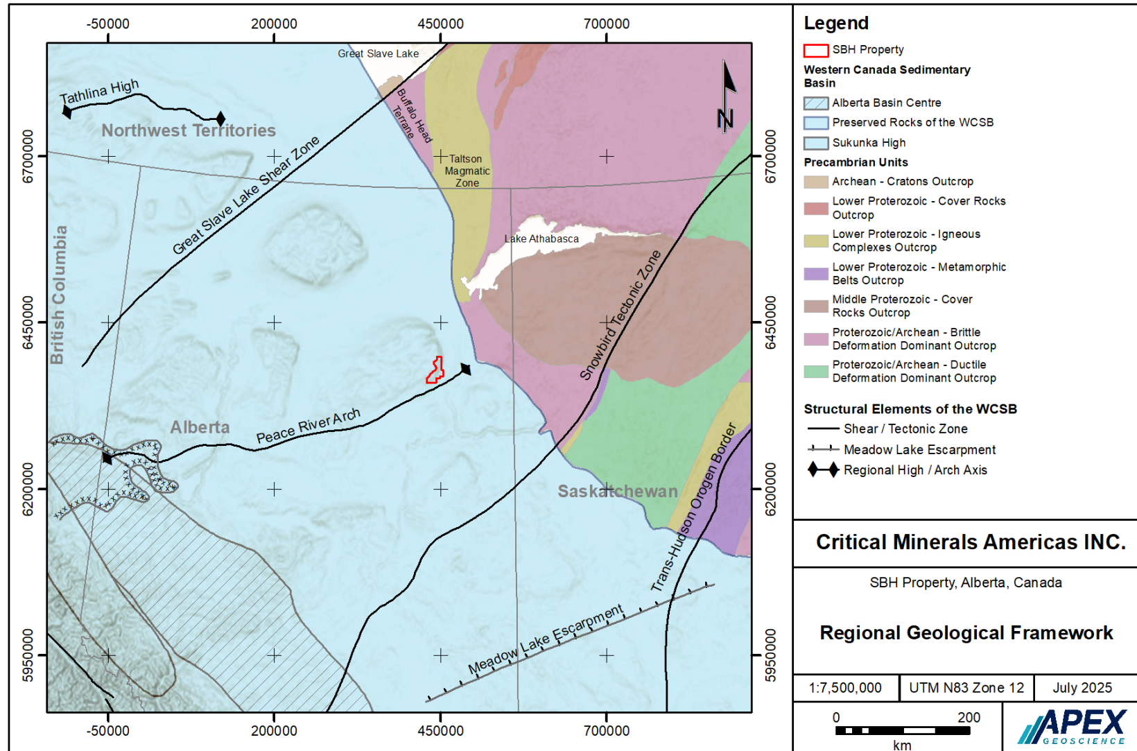
Figure 7.1 Regional geological framework of CMAI's SBH Property
