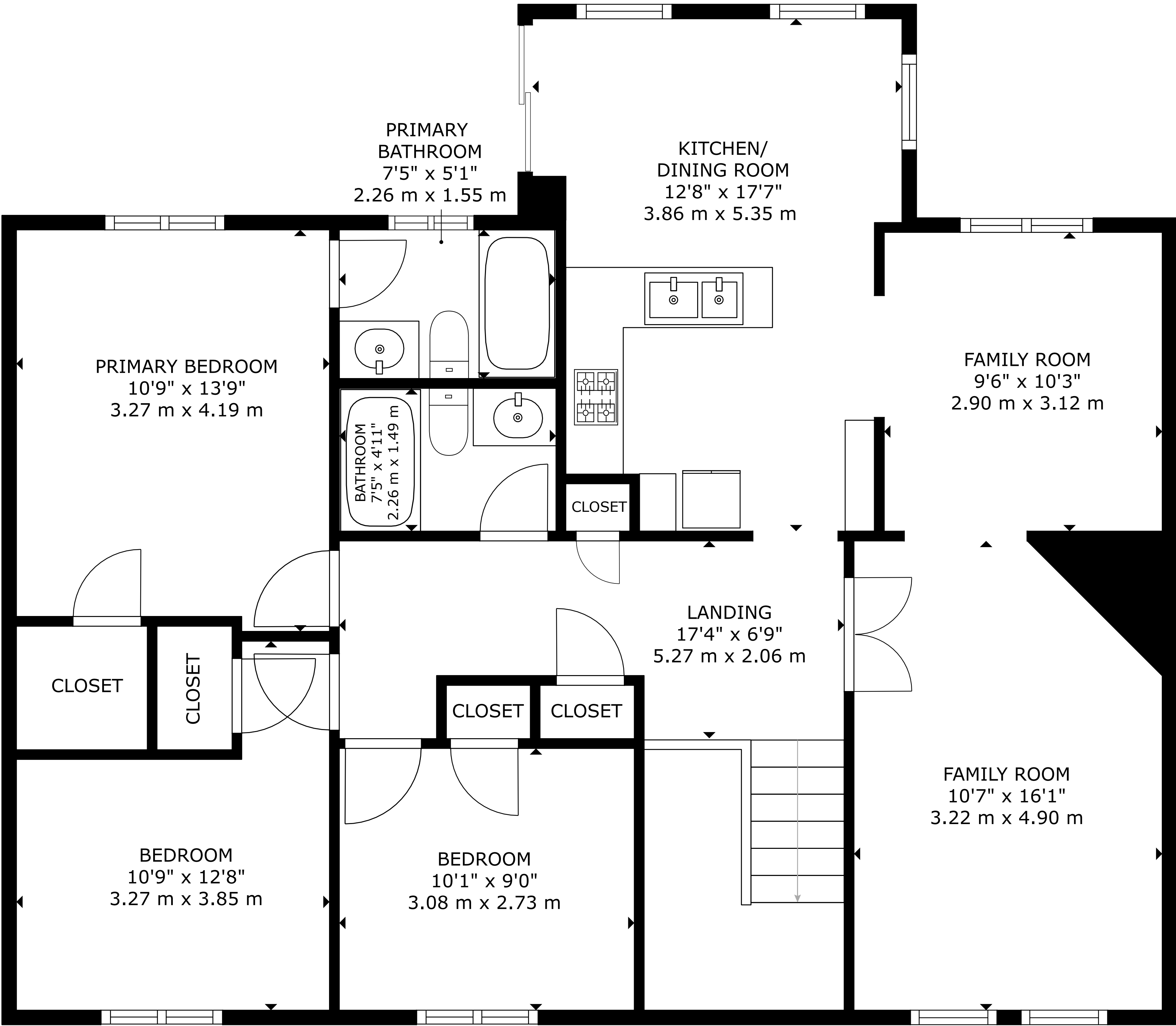
FLOOR 2
