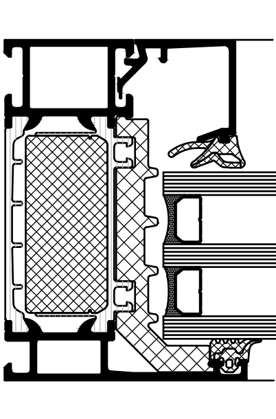
Horizontal section detail of Schüco Window System AWS 90.SI+
