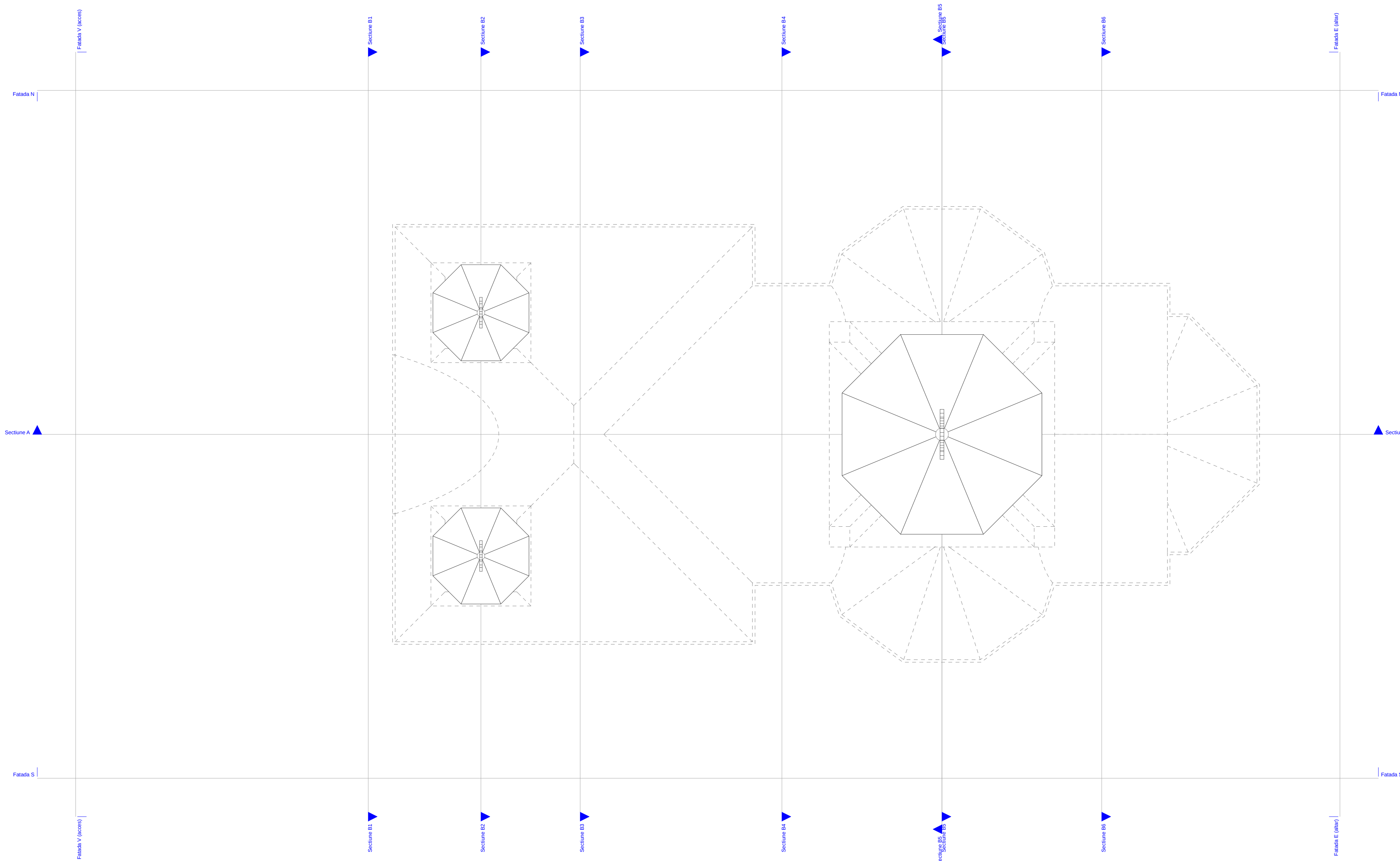
plan invelitoare turle sc. 1:100 belfries roofs plan sc. 1:100
