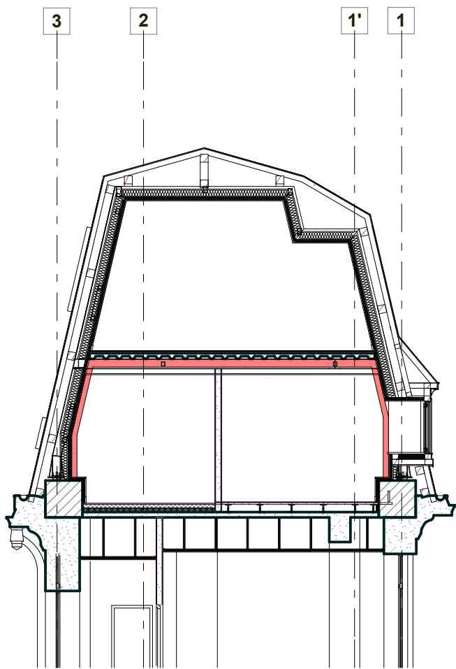
SECTION C-C
