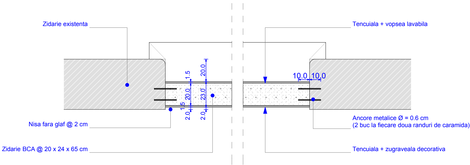
PLAN
