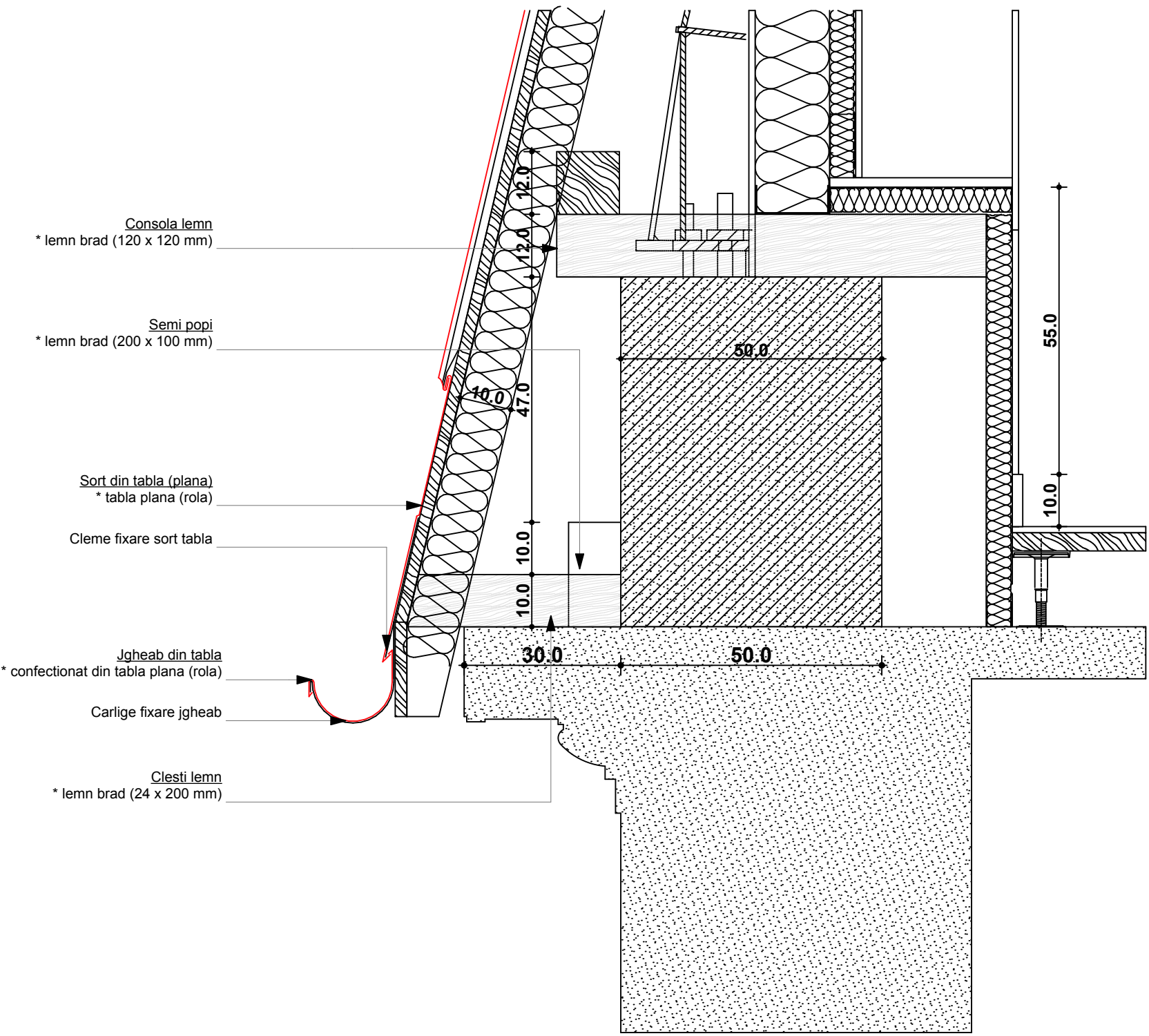
DETALIU STREASINA SPATE - TIP 2
