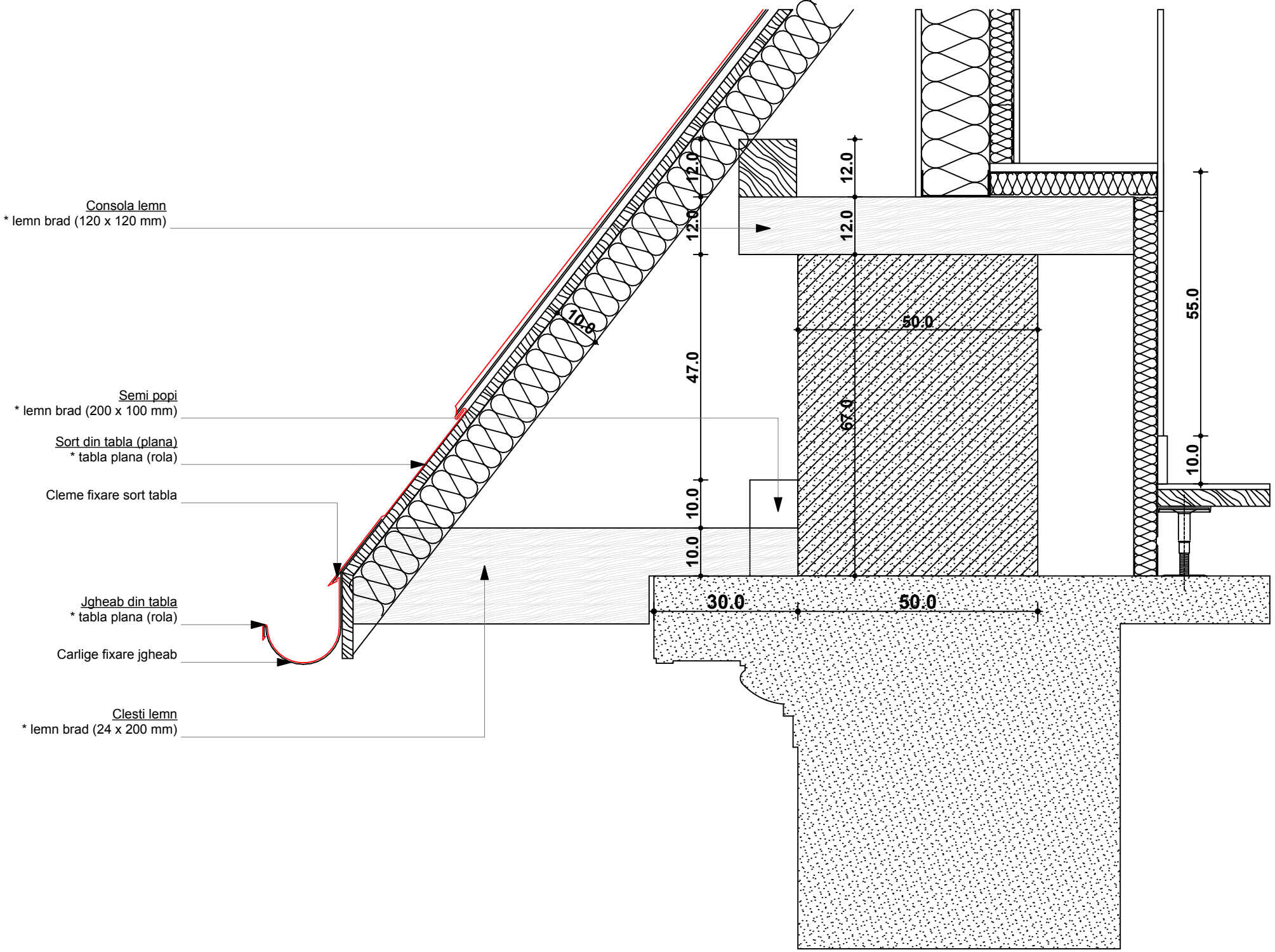
DETALIU STREASINA SPATE - TIP 1
