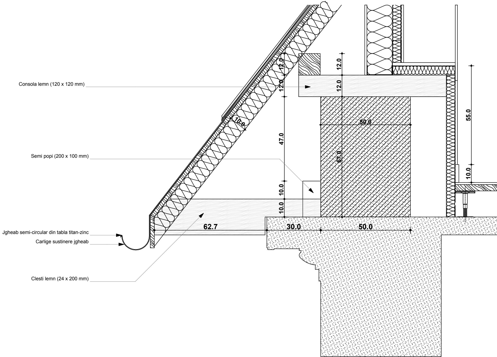
DETALIU STREASINA SPATE - TIP 1
