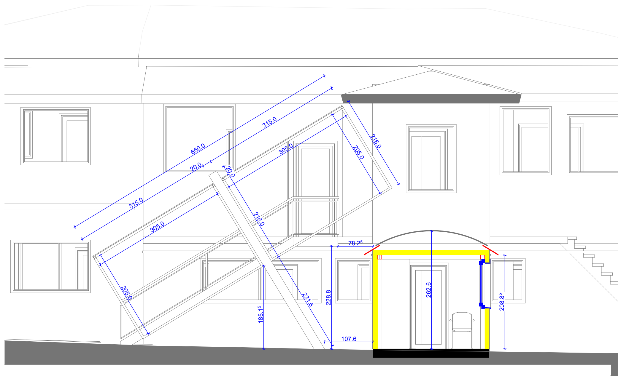
SECTION A
