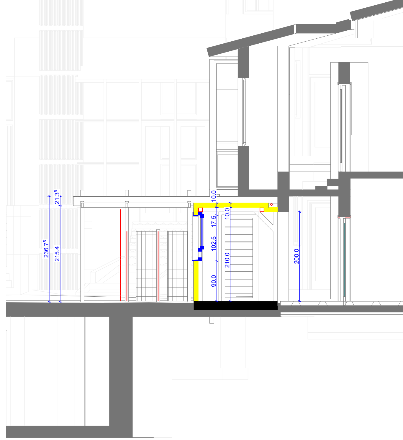
SECTION B
