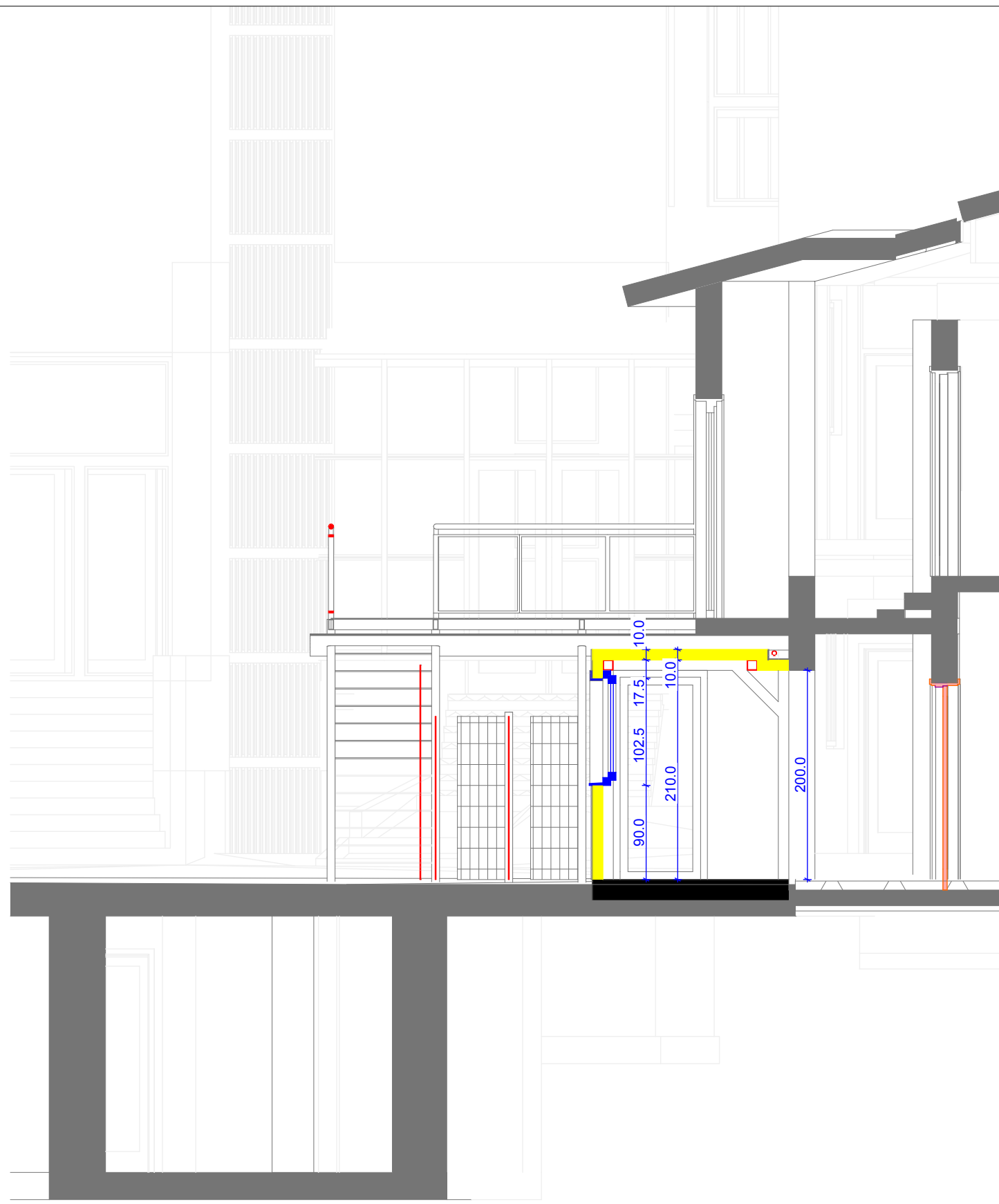
SECTION B
