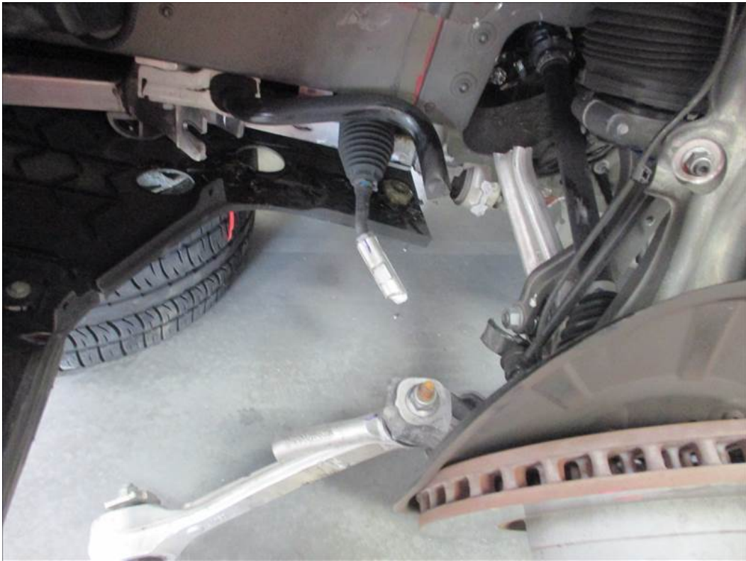
Steering gear
