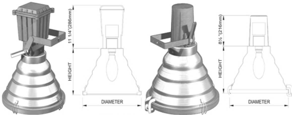
FORMED ALUMINUM REFLECTOR, ANODIZED FINISH
