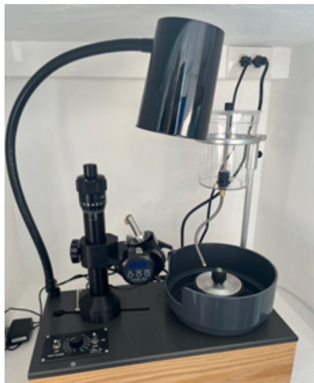
Ultra-Tec faceting machines are some of the best on the market. This model is the VL.
