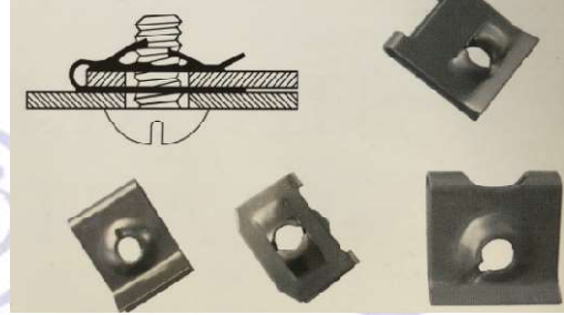
"U" NUTS-PRONG FORM AND KEYHOLE THREAD IMPRESSIONS
