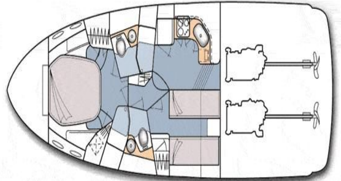
Manufacturer Provided Image: 400 - cabin arrangement
