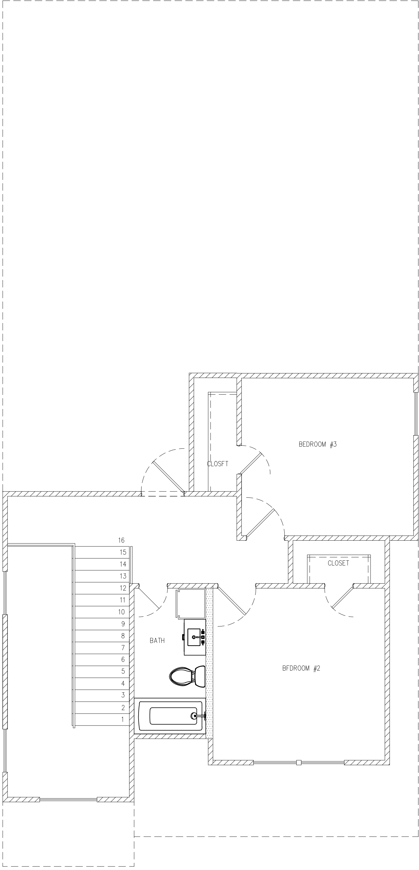
SECOND LEVEL FLOOR PLAN
