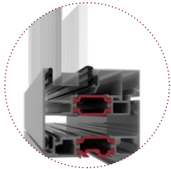
535 Casement Detail
