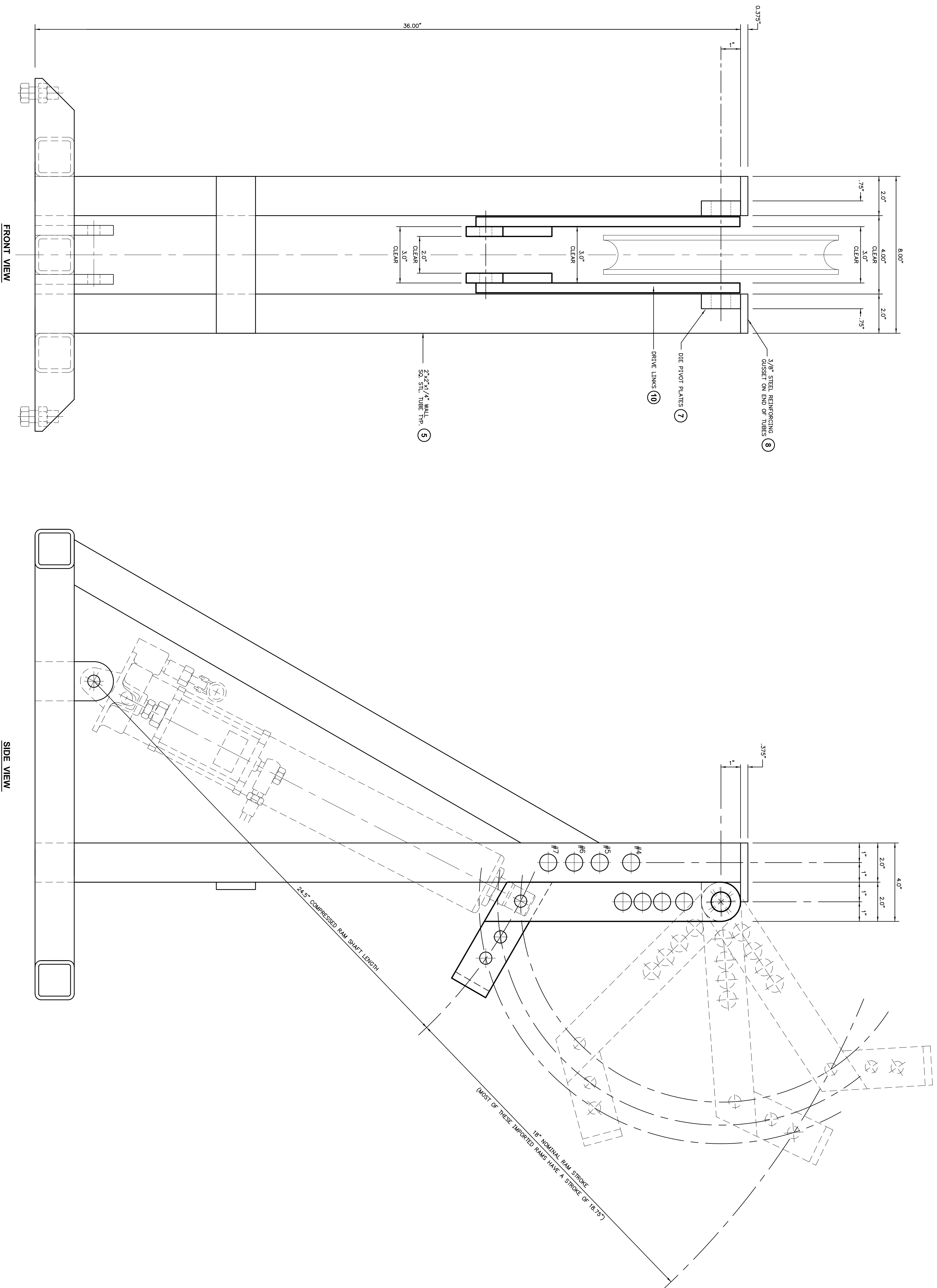
TYPICAL FRAME ASSEMBLY WITH DRIVE LINKS SCALE 1" = 1" (FULL SIZE)
