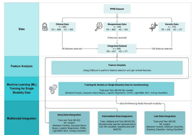
Fig. 2. Overview of the multimodal workflow used in the study.
