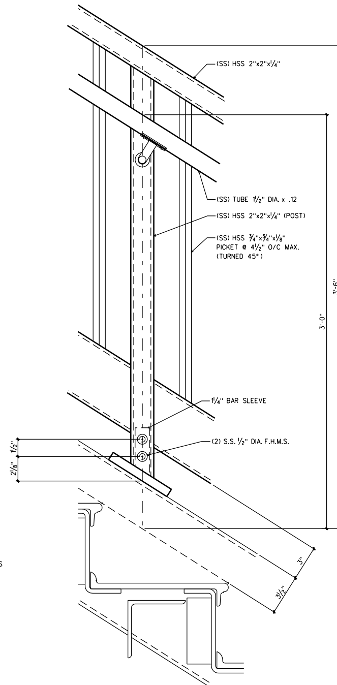
DETAIL "D3"
