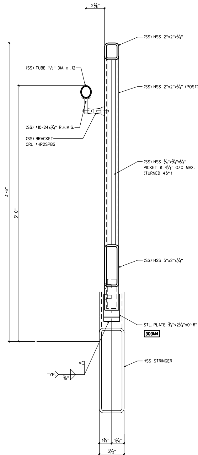
SECTION "7"
