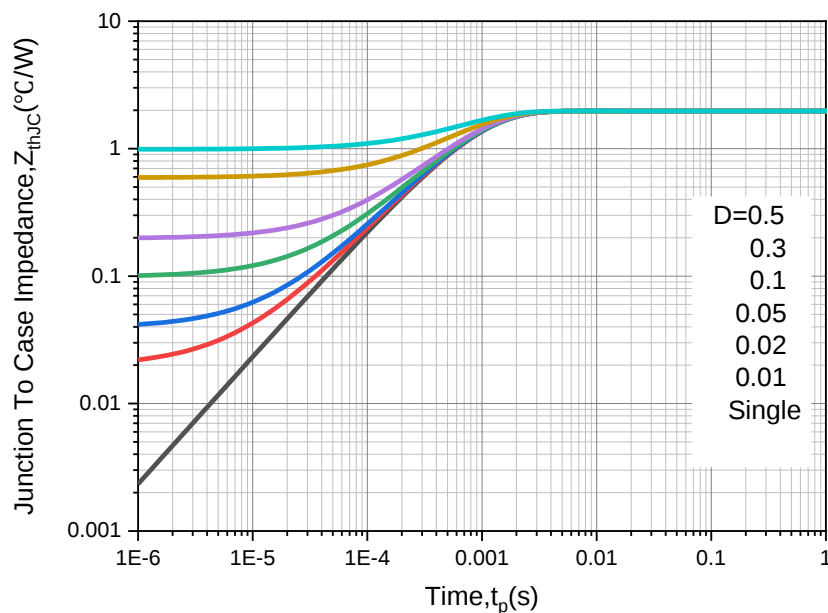
Figure 13. Transient Thermal Impedance (Junction-Case)
