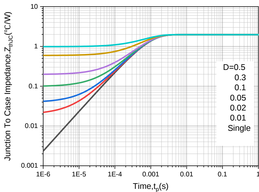
Figure 13. Transient Thermal Impedance (Junction-Case)
