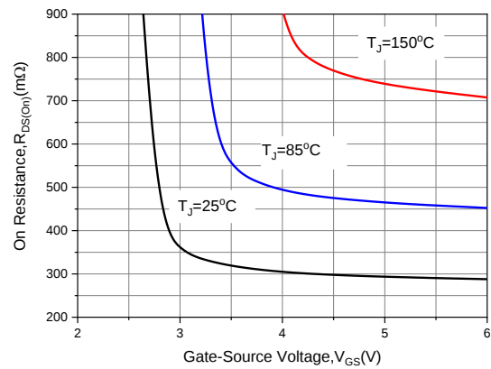
Figure 10. On-resistance vs. Gate Voltage @3A
