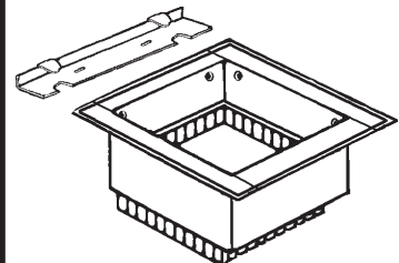
901990A ..... 6" Duct Connector 901991A ..... 8" Duct Connector
