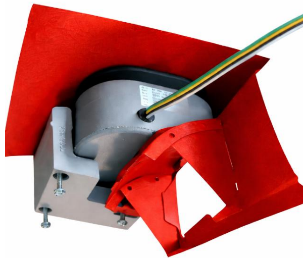
Figure 2 – Speaker Position
