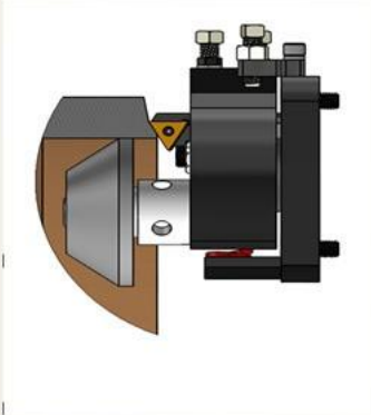
30° degree tool
