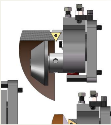
30° degree tool
