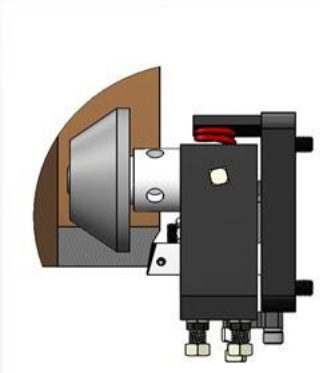
10° degree tool
