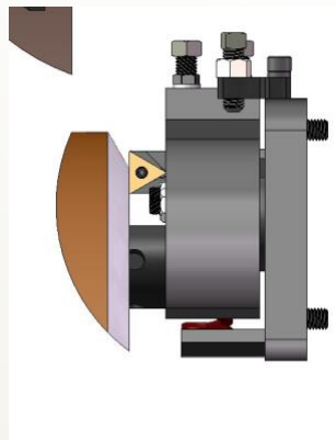
Land Tool
