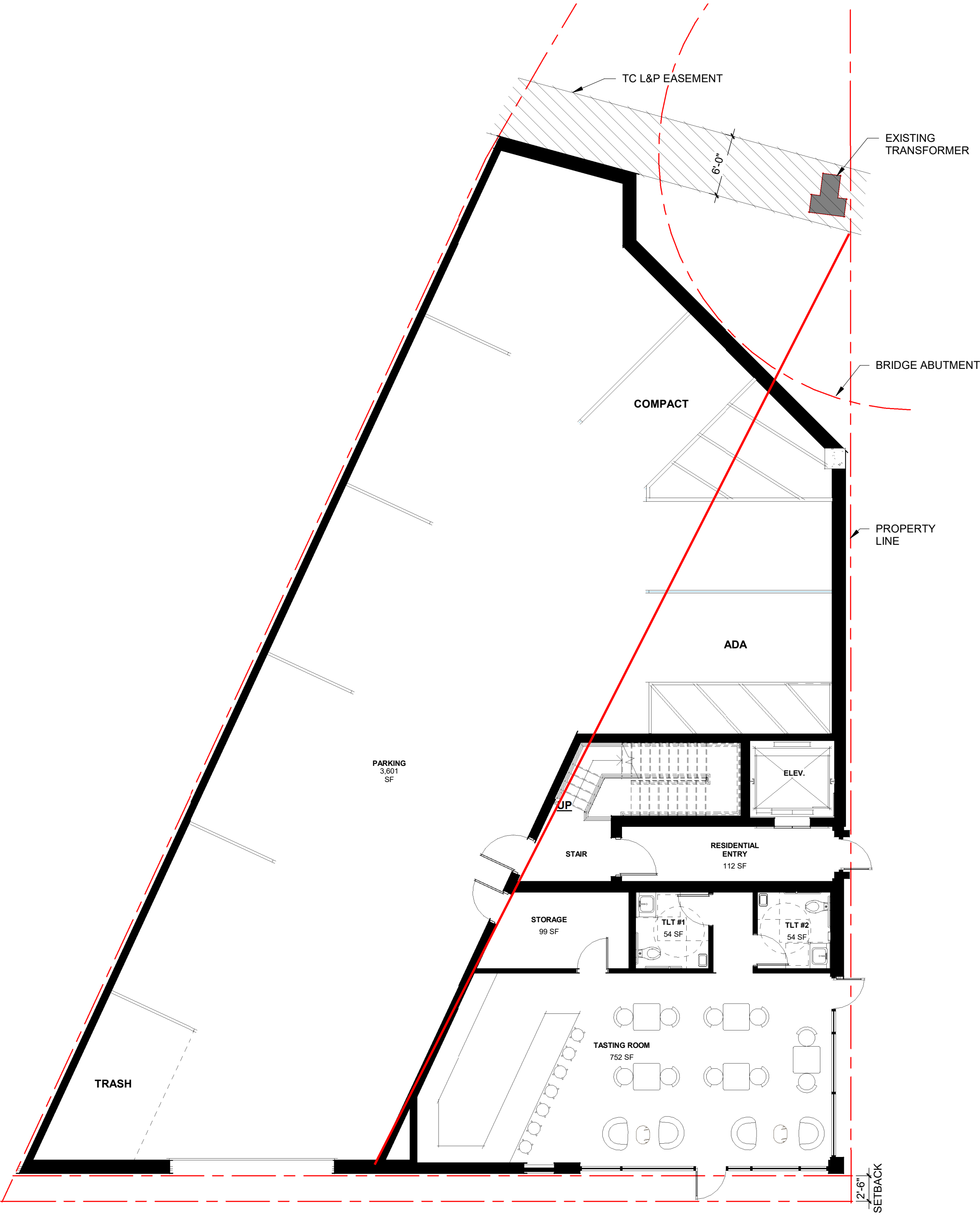
① FIRST FLOOR PRESENTATION PLAN 1/8" = 1'-0"
