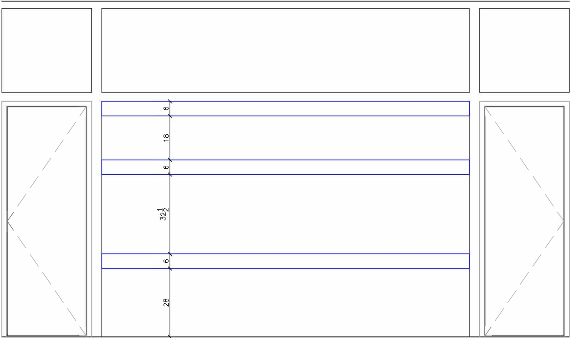
BLOCKING IN WALL FOR SHELVES / CABINETS
