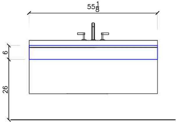
BLOCKING IN WALL FOR PRIMARY BATH VANITY
