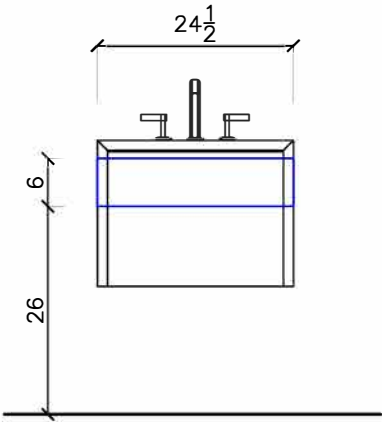
BLOCKING IN WALL FOR GUEST BATH VANITY
