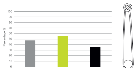
Fig.: Tensile strength clove hitch as a percentage of the original strength of the sewn sling.
