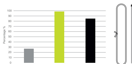
Fig.: Tensile strength tape knot as a percentage of the original strength of the sewn sling. * Dyneema® slips at about 5 kN and therefore may not be knotted.
