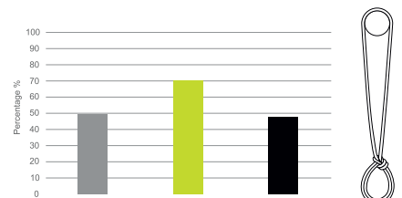
Fig.: Tensile strength double bowline as a percentage of the original strength of the sewn sling.
