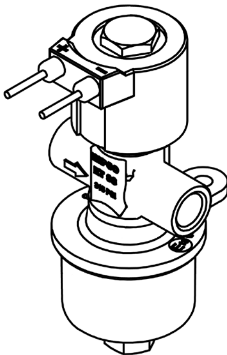
ET98 Fuel Lockoff, part number ET98-51315-001
