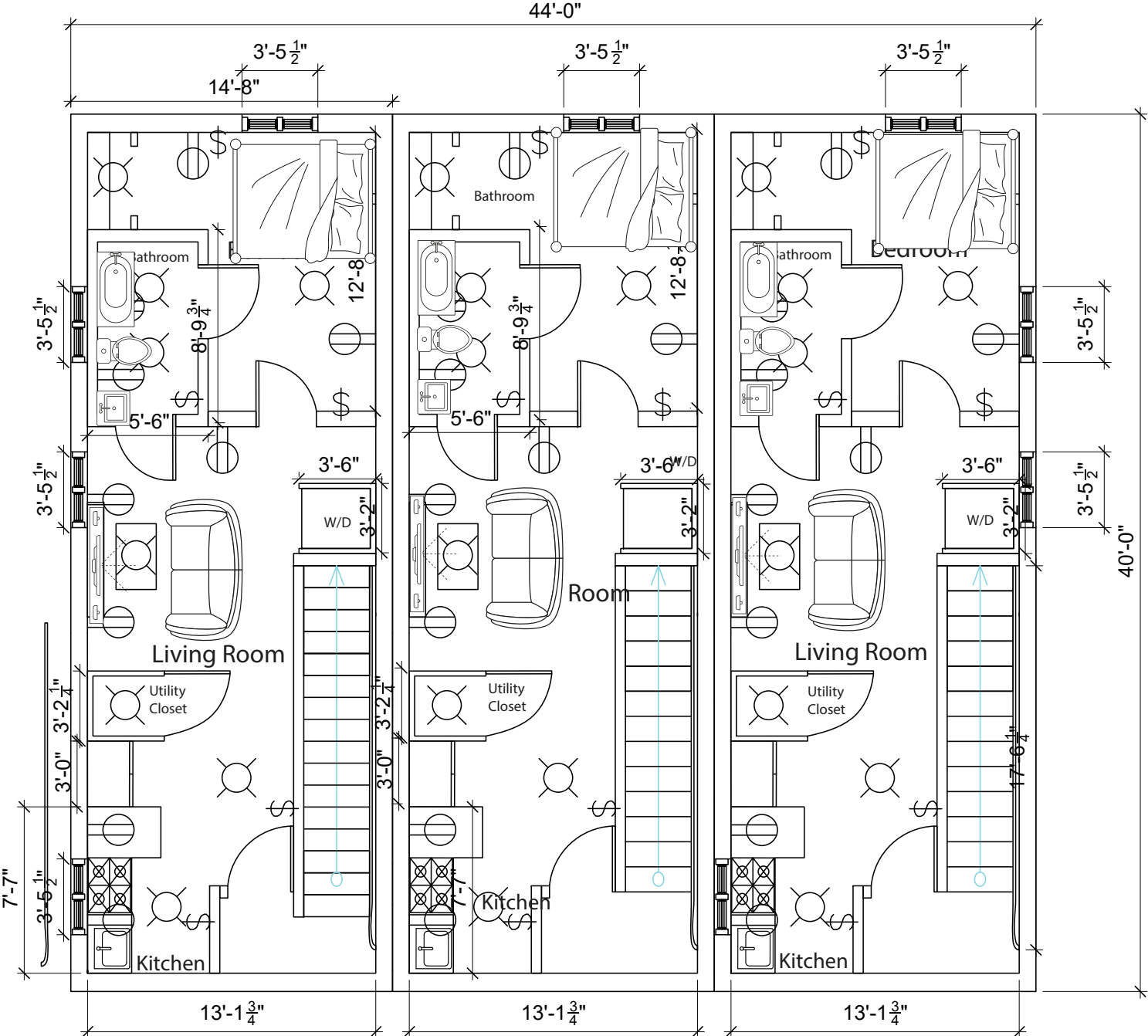
First Floor
