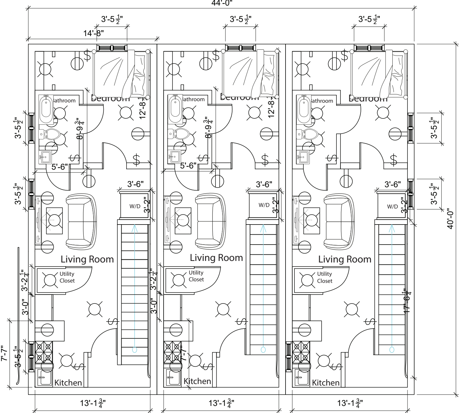
Second Floor
