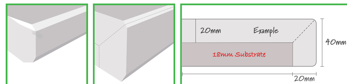
Square Aris 20mm & 40mm edge profile Natural Stone
