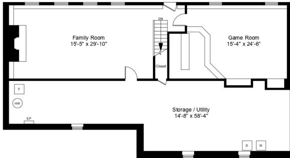
Lower Level Plan Ceiling Height = 6'-10"
