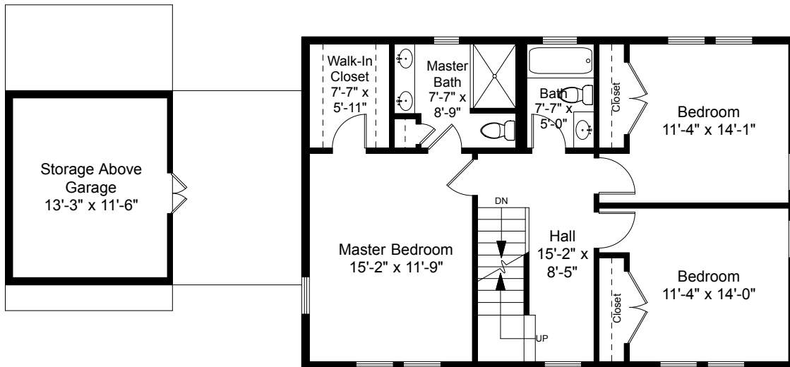
Second Floor Plan Ceiling Height = 7'-10"
