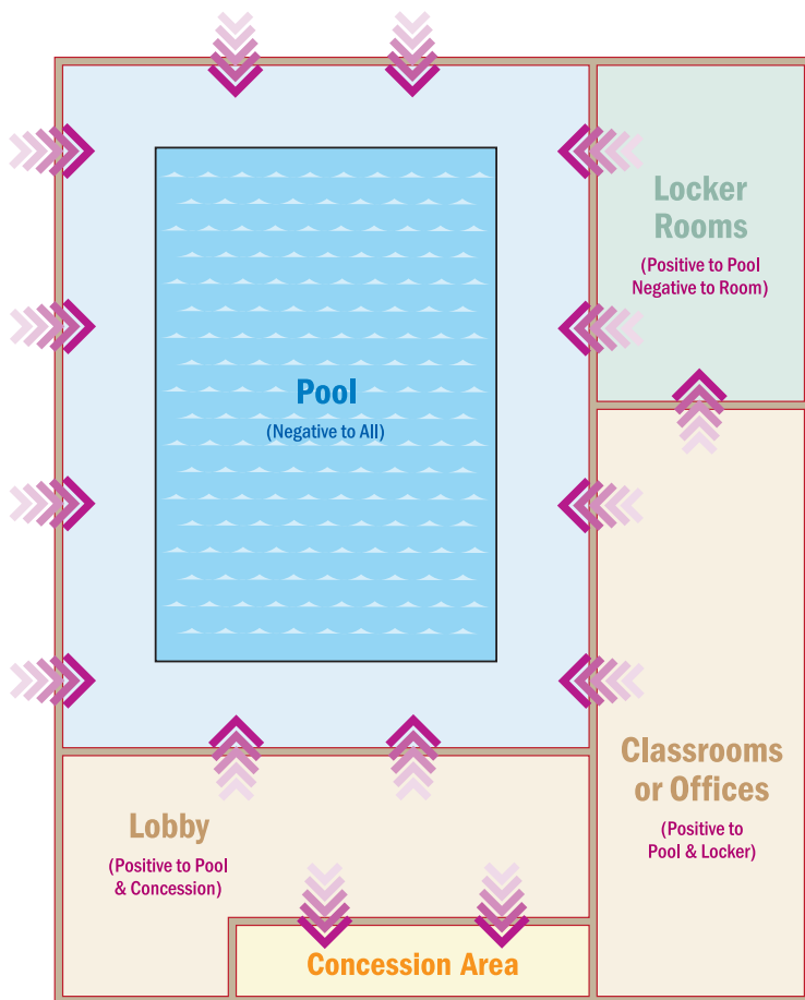
Figure 6. Building pressurization.
