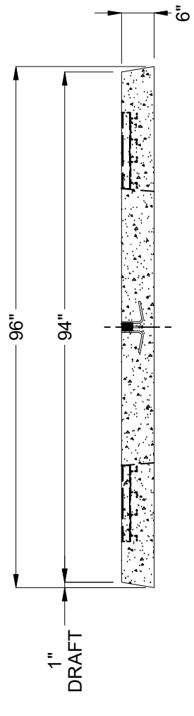
SECTION B-B
