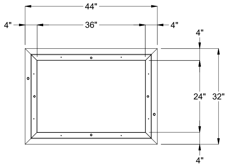
PLAN VIEW OF TOP SECTION
