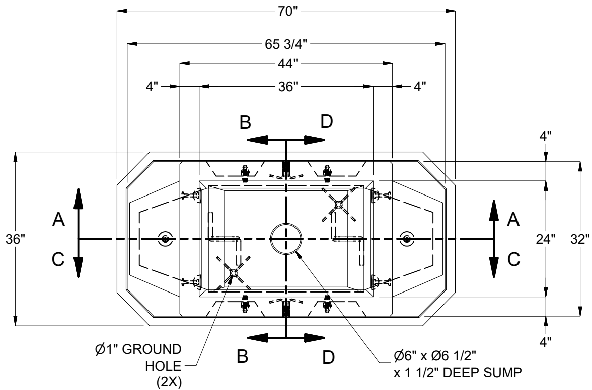
PLAN VIEW W/O TOP SECTION
