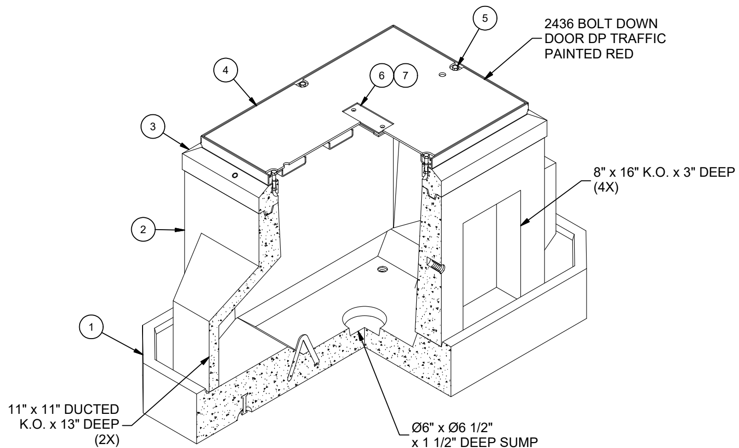
ISOMETRIC VIEW
