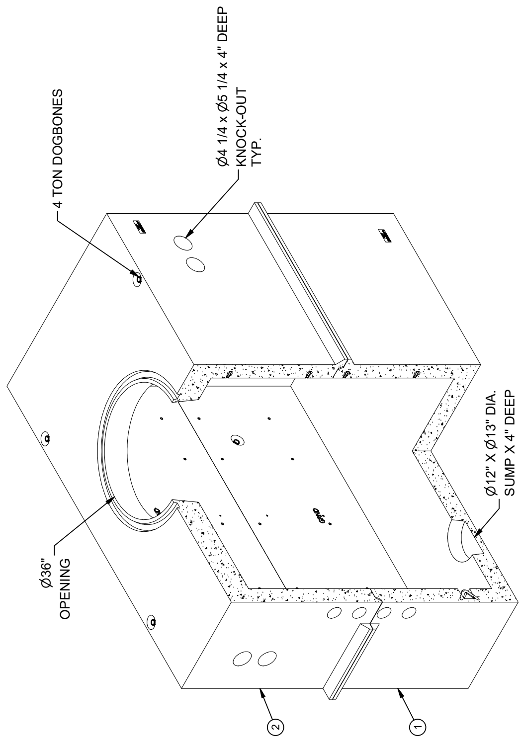
ISOMETRIC VIEW
