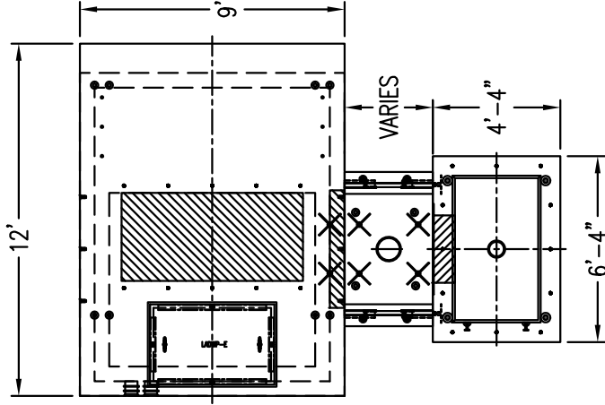
PLAN-VIEW G1-EXAMPLE
