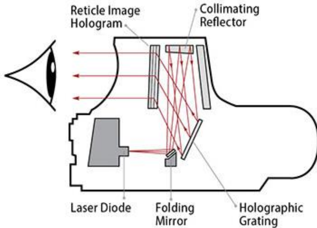
Holographic Laser Projection Optic
