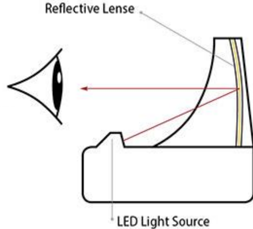
Reflex / Red Dot Sight (RDS) with LED Diode Emitting Optic
