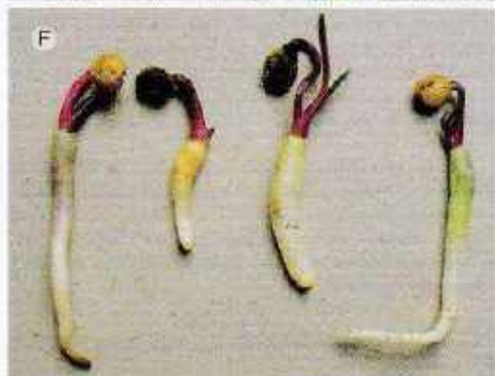
Plate 1. Clivia mirabilis , A, inflorescence in habitat showing orange/red pedicels; B, plants in habitat between Peninsula Formation Sandstone boulders; C, leaves showing prominent median white stripe on upper surface and variation in dimensions. D, E, fruiting head; D, immature berries; E, mature berries; F, seedlings five months after germination, note large radicle and prominent carmine pigmentation on cotyledon and at base of first pair of leaves. Photo: C. Paterson-Jones.
