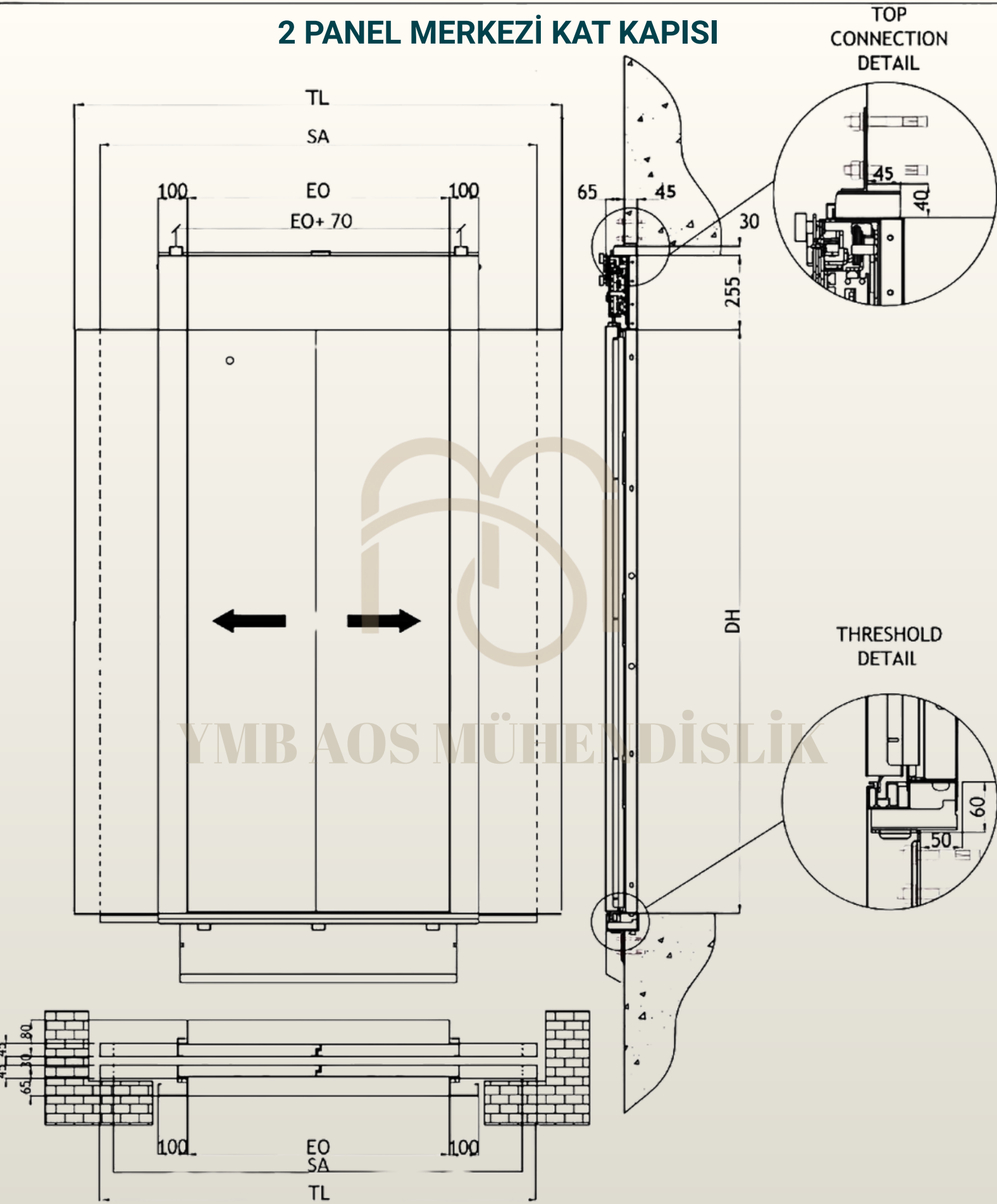
Technical Dimensions
