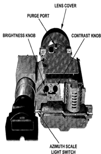
Figure 3-1: AN/KAS-1 Sensor Unit Controls (back view).
