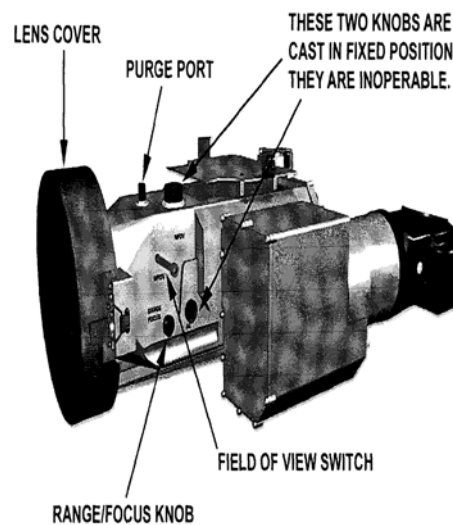
Figure 3-2: AN/ KAS-1 Sensor Unit Controls (side view).
