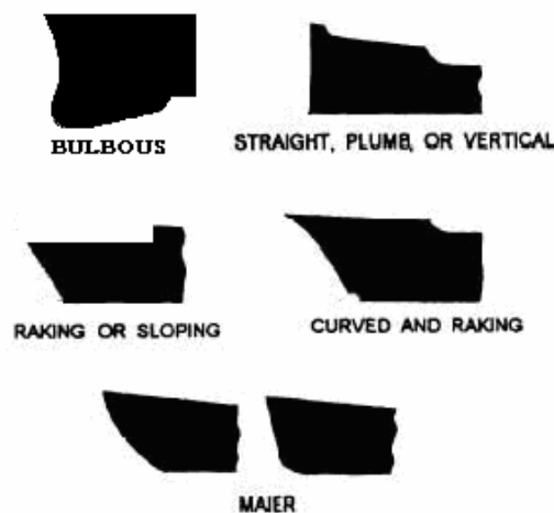
Figure 11-12 Bow Designs.
