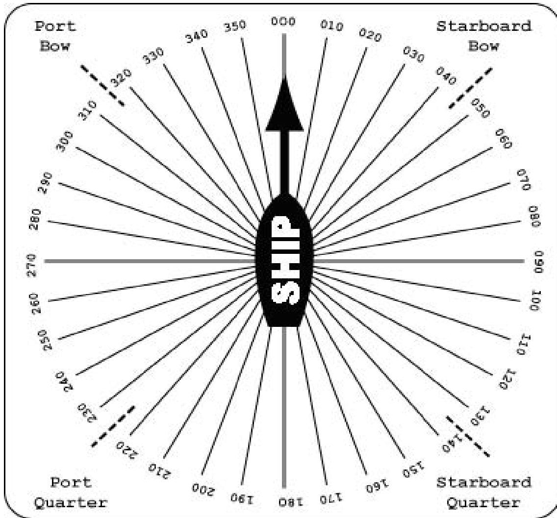
Figure 5-1: Relative Bearing.
