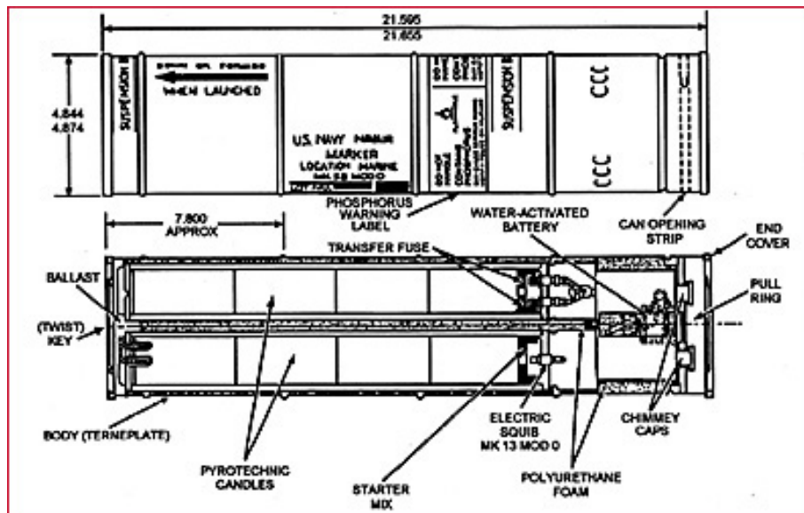
Figure 6-2: Mk 58 Marine Location Marker.
