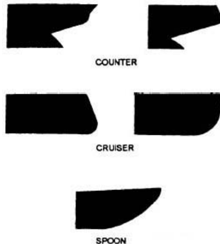
Figure 11-13 Stern Designs.
