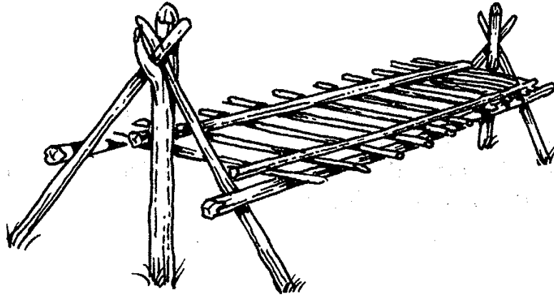
A camp bed off the ground is supported by a triangle of stakes at both ends.
