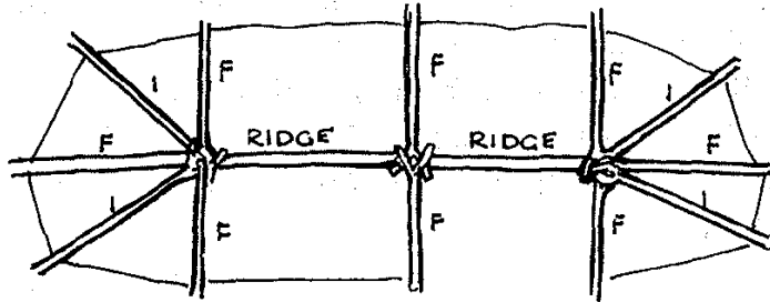
Basic structure plan of a long hut as seen from above. Intermediate support poles are needed for the ridge if the forks are more than 2 metres apart.
